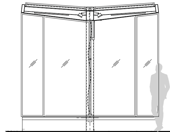
6 SIDE ELEVATION SCALE: 1/4" = 1' - 0"
