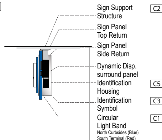
4 FACE LAYOUT - SOUTH SCALE: 1/2" = 1' - 0"
