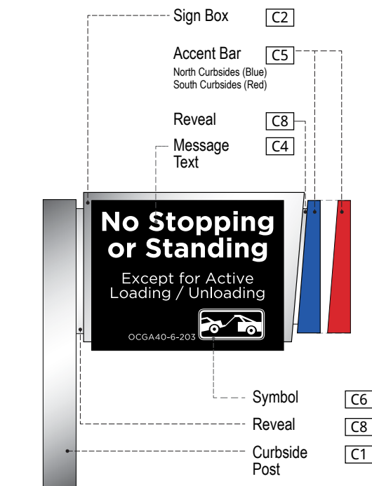
3 SIGN FINISHES SCALE: NTS
