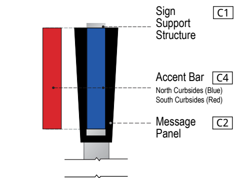
2 SIGN FINISHES SCALE: NTS
