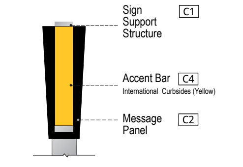
2 SIGN FINISHES SCALE: NTS
