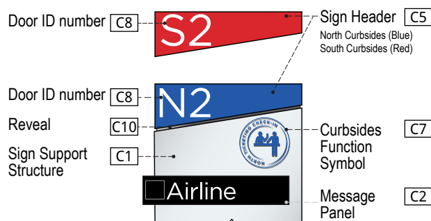
2 SIGN FINISHES SCALE: NTS
