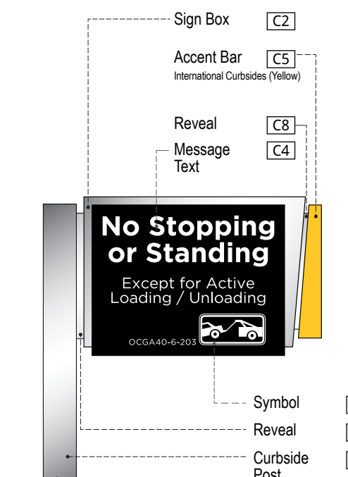
3 SIGN FINISHES SCALE: NTS
