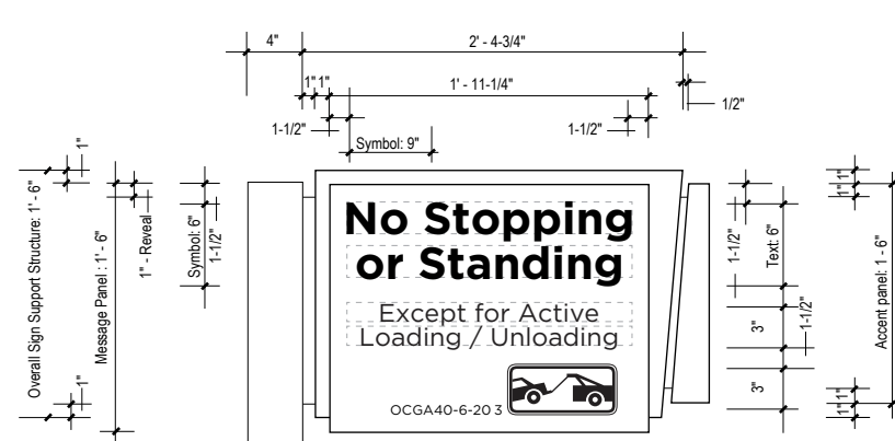
1 FINISH - TOP VIEW SCALE: NTS
