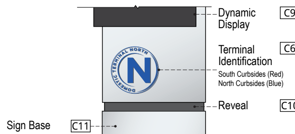
3 SIGN FINISHES SCALE: NTS
