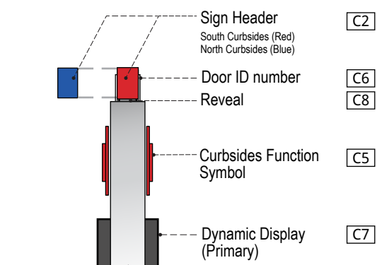
6 SIGN FINISHES - SIDE VIEW 2 SCALE: NTS
