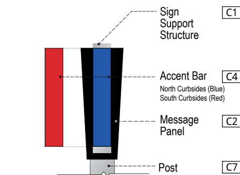
2 FINISH - END VIEW SCALE: NTS
