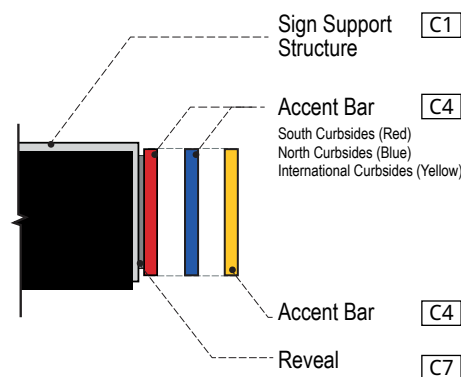
2 SIGN FINISHES SCALE: NTS
