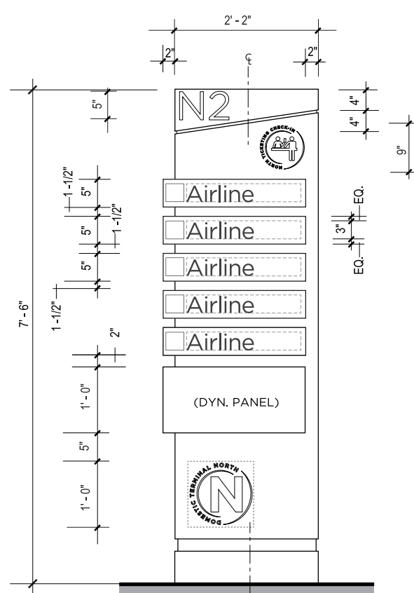
9 FACE VIEW SCALE: NTS
