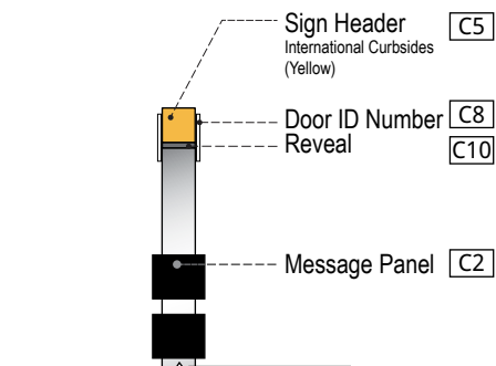
6 SIGN FINISHES - SIDE VIEW 2 SCALE: NTS
