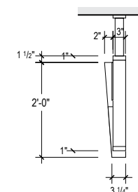
5 SIDE VIEW SCALE: 1/2" = 1' - 0"
