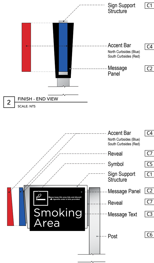
2 FINISH - END VIEW SCALE: NTS
